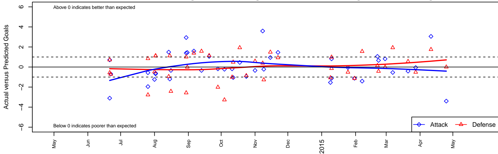
NWN Red B01 Dots are actual minus expected GF (blue circles) and GA (red triangles). Blue line is smoothed change in attack strength. Red is smoothed change in defense strength.
